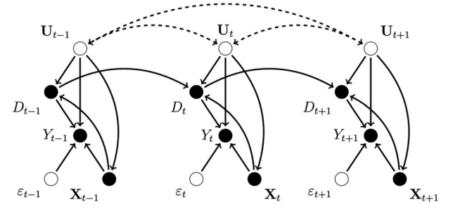
FIGURE 1 A DAG Illustration
